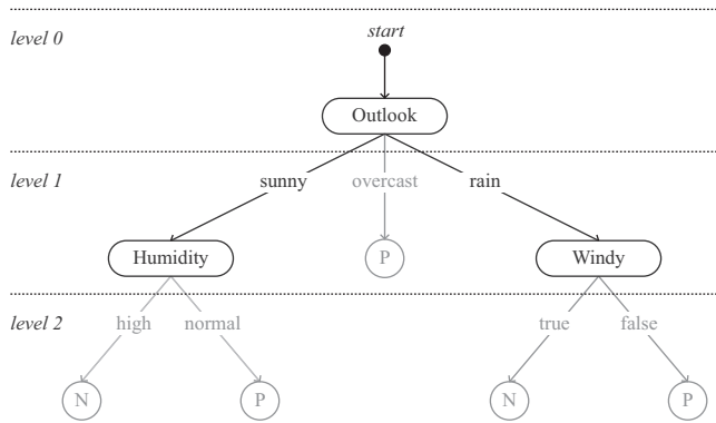
Fig. 6. An example of a decision tree created by an ant; the 'start' node represents the starting vertex. The highlighted branches—the branches that lead to a decision node, including the root node—are the ones that eventually will be used to update the pheromones. Branches whose terminal node is a leaf node, such as branches at level 2 in the figure, are the result of the deterministic pruning procedure or the case when all examples following the branch are associated with the same class label, therefore they are not represented in the pheromone matrix.
