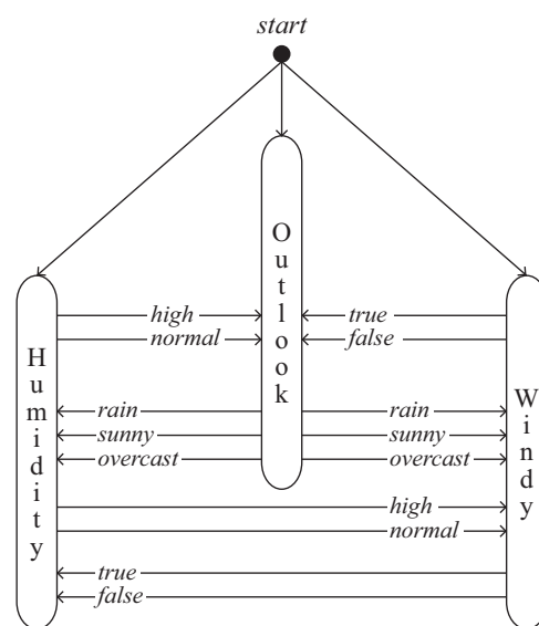
Fig. 4. An example of a construction graph that can be used to generate the decision tree presented in Fig. 1. In this example, the construction graph is composed by three vertices representing nominal attributes: Outlook {sunny, overcast, rain}, Humidity {high, normal} and Windy {true, false}; and a virtual 'start' vertex.
