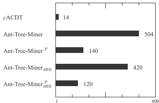
Fig. 7. Average computation time (over all data sets) in seconds to complete a fold of the cross-validation for each of the ACO-based algorithms on a 3.33 GHz Intel Xeon computer. The deterministic C4.5 and CART algorithms take on average 1 second to complete a fold of the cross-validation.
