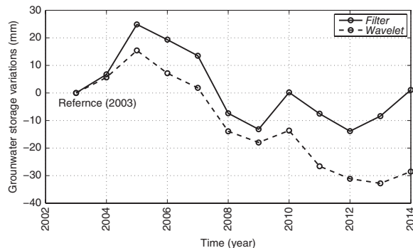
Figure 10. The time histories of groundwater storage variations with a respect to 2003 as a reference year.
