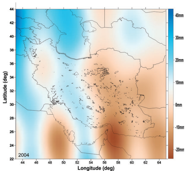
Figure 7. Groundwater storage variations related to Equation 8 based on Gaussian filtering in 2004.
