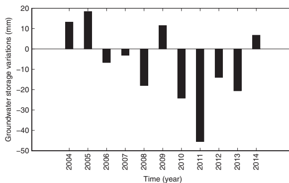
Figure 11. Mean variations amplitude of groundwater by wavelet over Urmia Lake.
