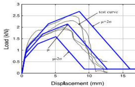
(b) fastener strength and fastener test curve
