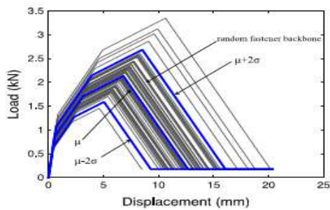
(c) brittle random fastener backbone model
