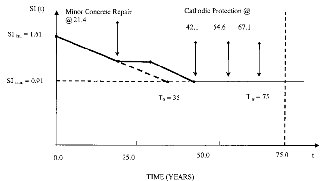
Fig. 7. Bridge safety index profile from one realization of Monte Carlo simulations
