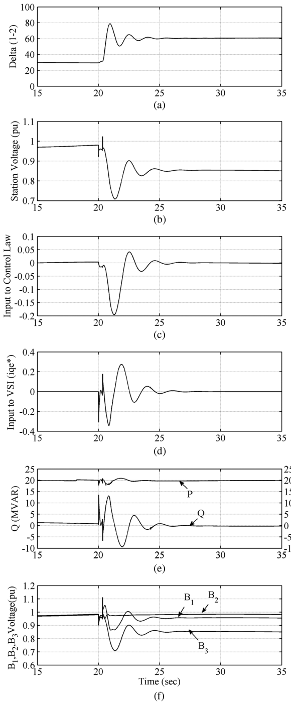
Fig. 5. Simulation results for the proposed control strategy corresponding to an L-G fault: (a) power angle between buses 1-2; (b) PV station voltage; (c) input to the control law after low-pass and washout filters; (d) reference current generated by the controller for reactive power component of current; (e) actual reactive and active power injection by the PV station, and (f) power system bus voltages.
