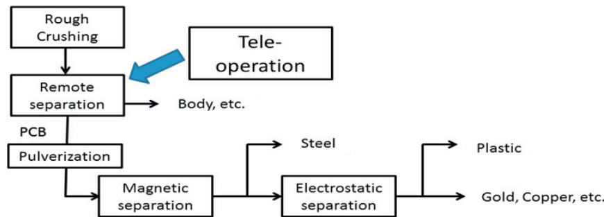
Fig. 10. Basic block diagram of a recycling process including remote separation
