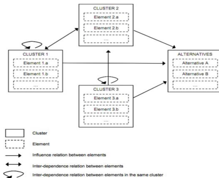
Fig. 12: Example of network structure with clusters and elements Source: Bottero et al., 2007
