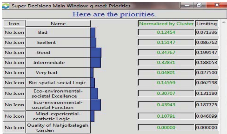
Fig. 17: Final vector with global priority deriving from limited matrix Source: Authors
