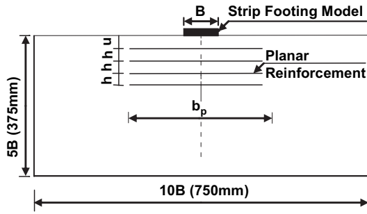
Fig. 5. Geometry of the planar reinforced foundation bed.
