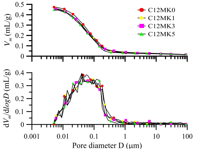
Fig. 6. MIP results of stabilized soils with 12% cement content.
