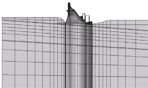
Figure 1 Finite element model of powerhouse dam section
