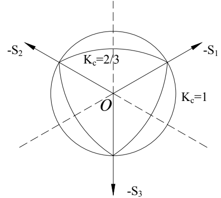
Figure 4 yield surface in the deviatoric plane with different values of K_c
