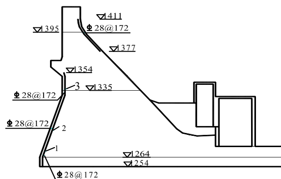
Figure 2 Typical dam section
