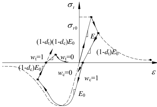
Figure 3 Stress-strain relationship of concrete under cycle loads
