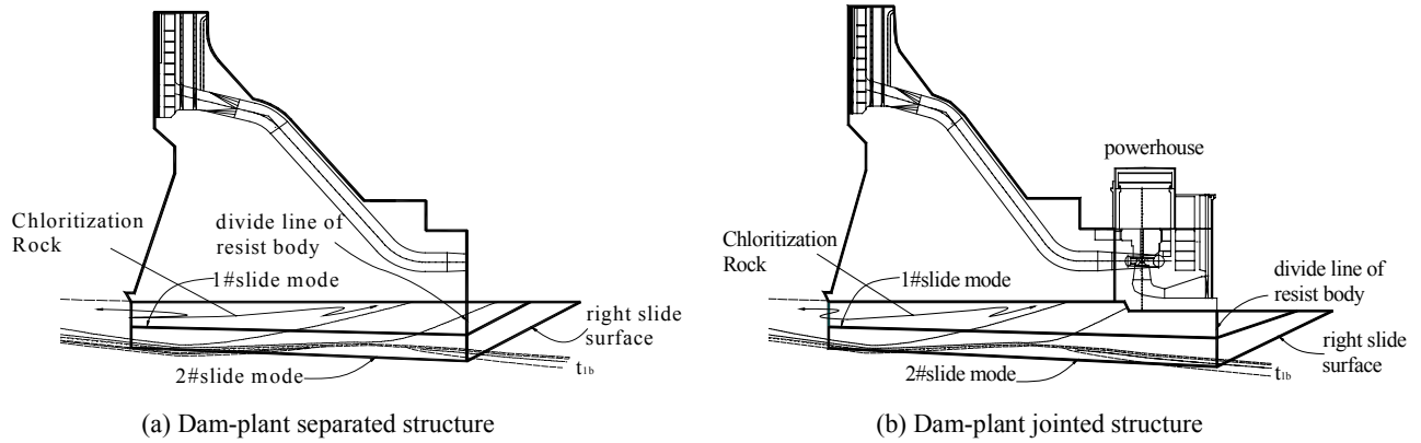
Figure 10 Deep sliding modes of the powerhouse dam section
