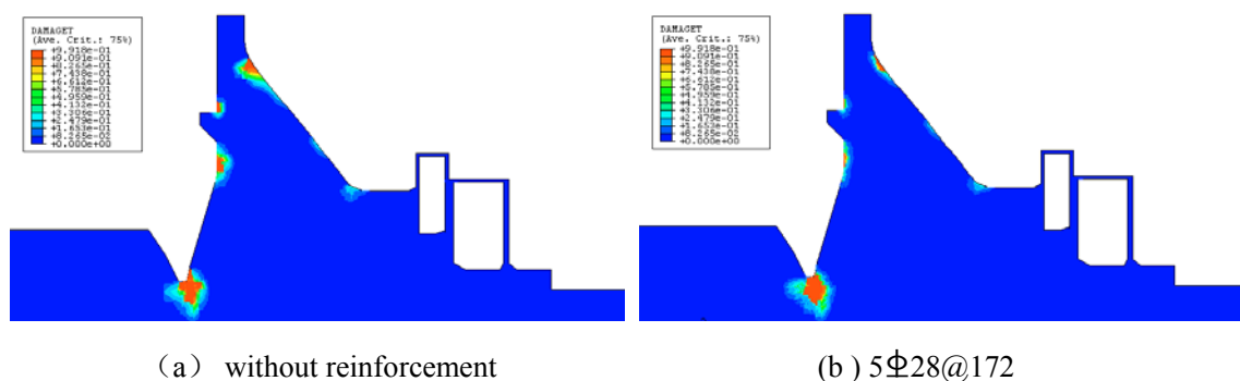
Figure 7 Damage cracking depth of dam
