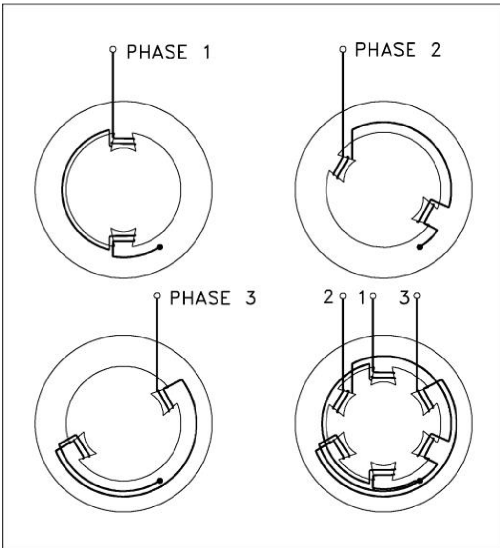
Figure 1 Three-Phase Stator
