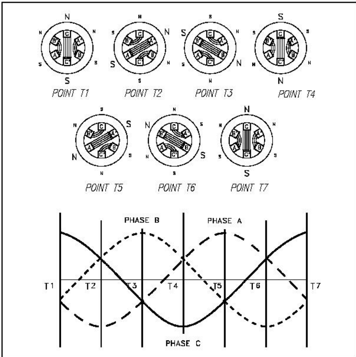
Figure 2 Rotating Magnetic Field
