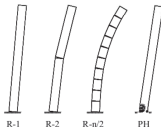
Fig. 5. Schematic representation of considered rocking sections and plastic hinge models.
