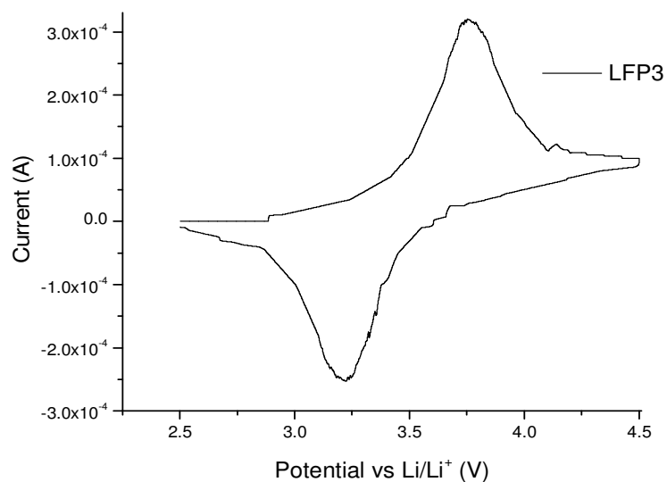
Fig. 3. Cyclic voltammograms of LFP3 sample in the first cycle at a scan rate of 0.1 \text{ mV s}^{-1} between the potential limit of 2.5 and 4.5 V (vs. \text{Li}^+/\text{Li} )
