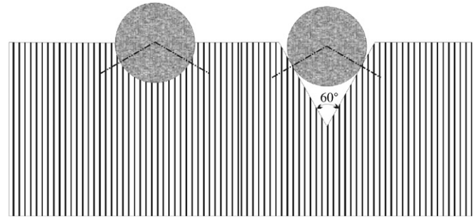
Fig. 3. Cross sections of steel-base blocks with the arc- and V-shaped machined slots in which NX size (54.7 mm) core specimens are seated. (While the use of V-shaped slots is discouraged, if used, the slots should have the specified angle to ensure identical seating positions for different diameter specimens. Also note that an arc angle of 120^\circ is sufficient for similar lateral confinement as in V-shaped slots.)
