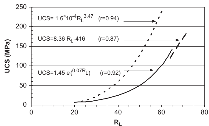
Fig. A1. Comparison of predictions of the uniaxial compressive strength ( UCS ) of granites based on their rebound hardness values ( R_L ) using the L-type hammer. (dotted: [7]—Grade I–IV; dashed: [8]—Grade I; solid: [2]—Grade I–IV).
