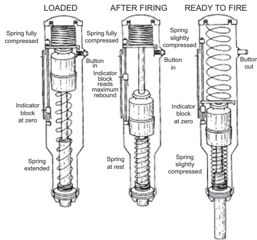
Fig. 1. Working principle of a Schmidt hammer [3].
