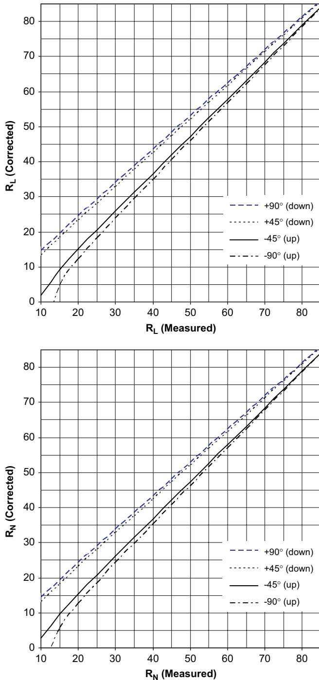
Fig. 2. Normalization of rebound values obtained by (a) L- and (b) N-type Schmidt hammers at selected angles [4] (Positive and negative angles refer to the downward and upward positions of the SH, respectively).
