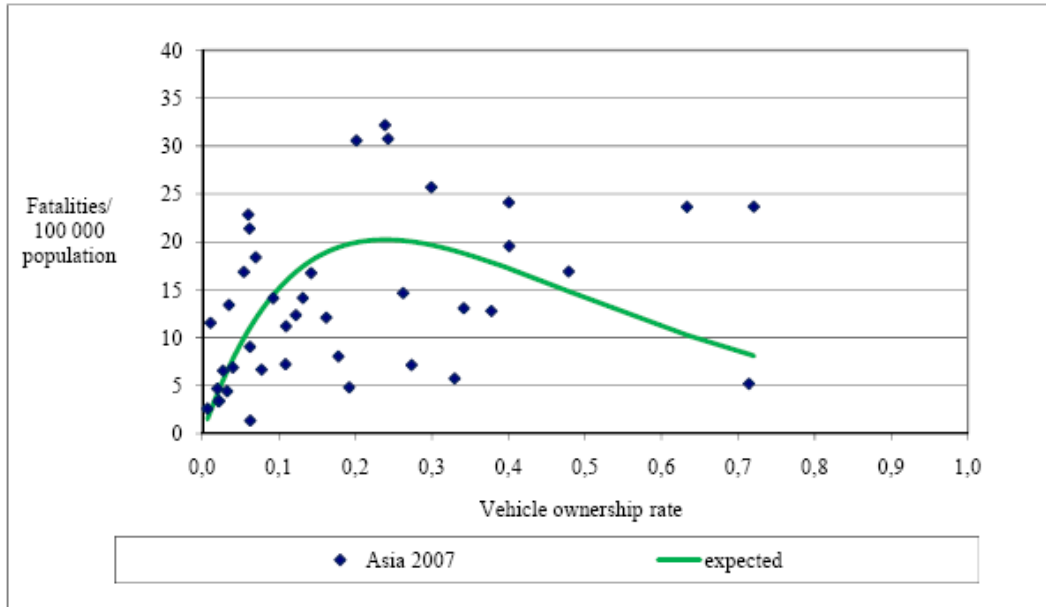
Figure 9. Relationship between vehicle ownership and fatality rate per population for Asia
