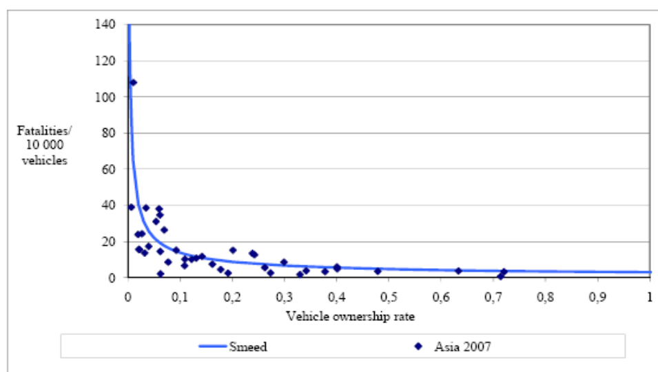
Figure 8. Relationship between vehicle ownership and fatality rate per vehicles for Asia
