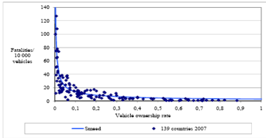
Figure 3. Vehicle ownership and fatality rate per vehicles in 2007 compared with Smeed
