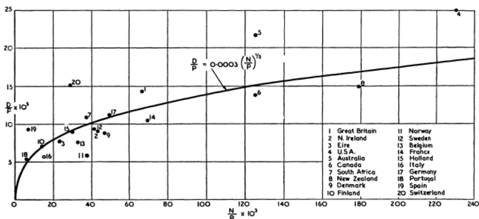
Figure 2. Relation between number of fatalities per 100 000 population and number of registered vehicles per 1 000 population for 1938
