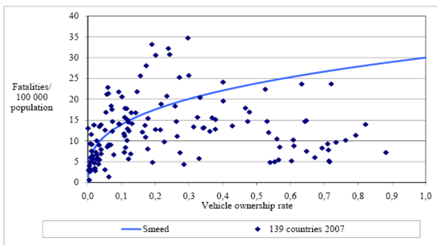
Figure 5. Vehicle ownership and fatality rate per population in 2007 compared with the Smeed formula
