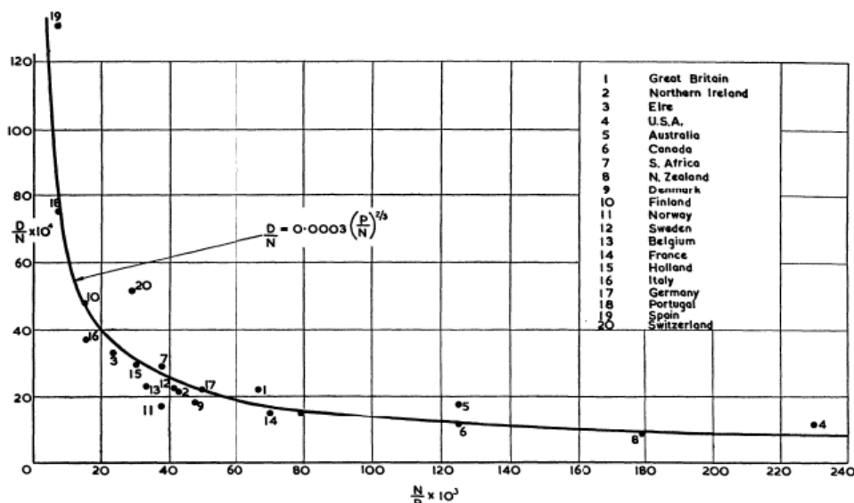
Figure 1. Relation between number of deaths per 10 000 registered motor vehicles and number of vehicles per 1 000 population for 1938
