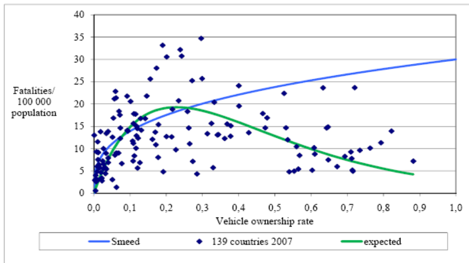
Figure 6. Relationship between vehicle ownership and fatality rate per population for 2007
