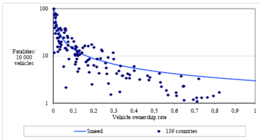
Figure 4. Vehicle ownership and fatality rate per vehicles in 2007 compared with Smeed (log scale)
