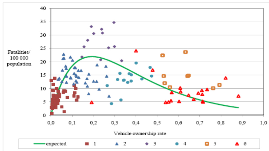
Figure 7. Clusters of countries according their GDP, ownership and fatality rates
