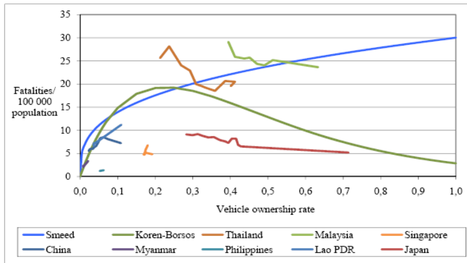
Figure 10. Changes of fatality rates versus vehicle ownership in some Asian countries
