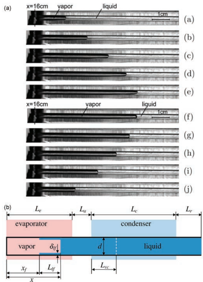
Fig. 17: (a) Visualization results for thermally driven meniscus oscillations by Das et al. [2010-a]. Consecutive snapshots of the transparent condenser showing the meniscus position for one cycle ( T_e = 45 °C, T_c = 10 °C and P_{res} = 90 kPa). Time interval between two consecutive images is 13.3 ms. The liquid reservoir is to the right, and the evaporator is to the left of the images. (b) Proposed model by Das et al. [2010-a].
