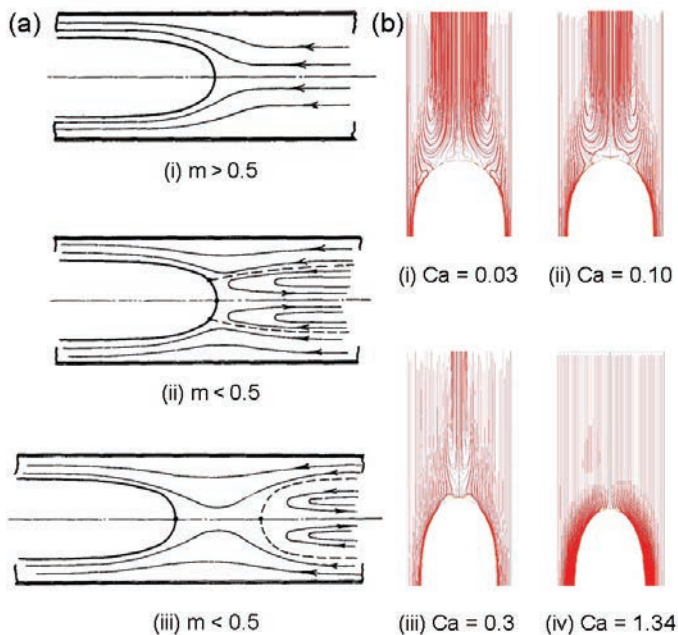
Fig. 7: Flow patterns in the liquid slug trapped between Taylor bubbles (a) as proposed by Taylor [1961] and (b) as numerically computed by Taha and Cui [2004].
