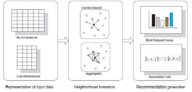
Figure 1 - Part of Recommendation Systems [4]
