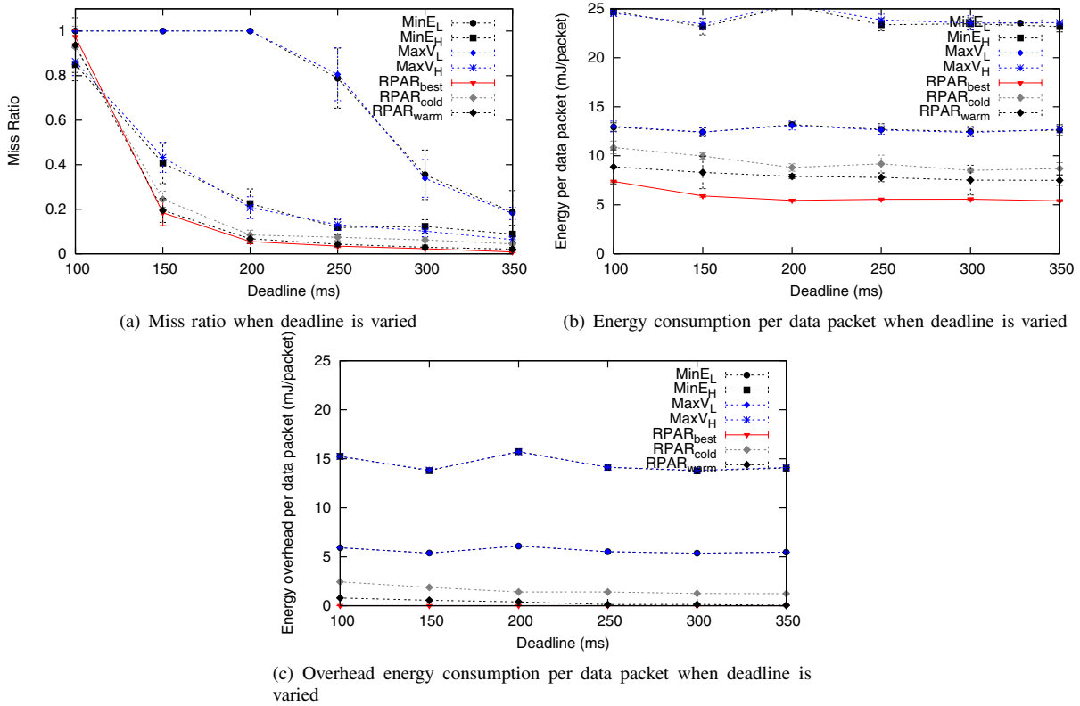
Fig. 3. Performance of considered protocols when deadline is varied (with neighborhood management).
