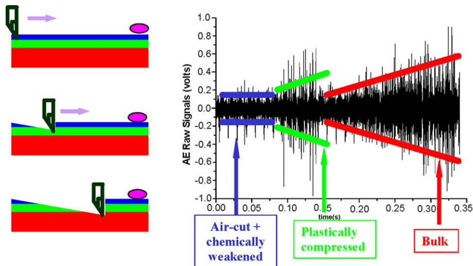
Fig. 10. Variation in AE RMS signal during scribing of CMP-treated oxide wafer.
