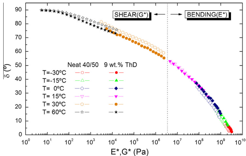
Fig. 5. “Black” diagram for neat bitumen 40/50 and its corresponding 9 wt.% ThD modified binder, after 60 days of curing.
