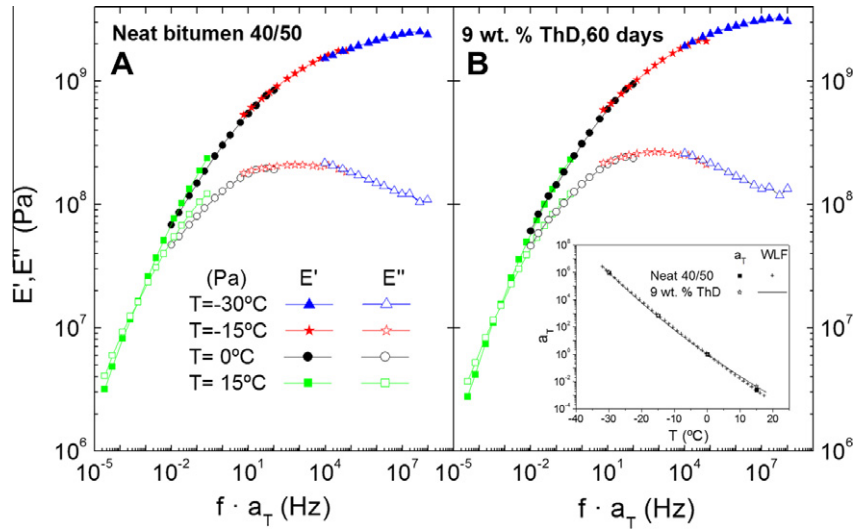
Fig. 4. Master curves of the linear viscoelastic moduli in dynamic bending, E' and E'' , for (A) neat bitumen 40/50 and (B) 9 wt.% ThD modified bitumen, after 60 days of curing. (Inset: Temperature dependence of the shift factor, and WLF fitting, for both binders.)
