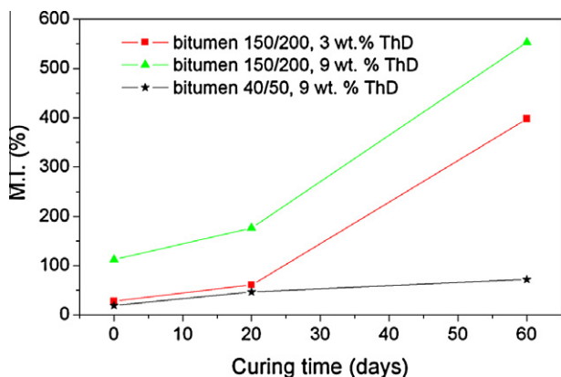
Fig. 2. Evolution of the modification index with curing time, for three selected ThD modified bitumen samples.
