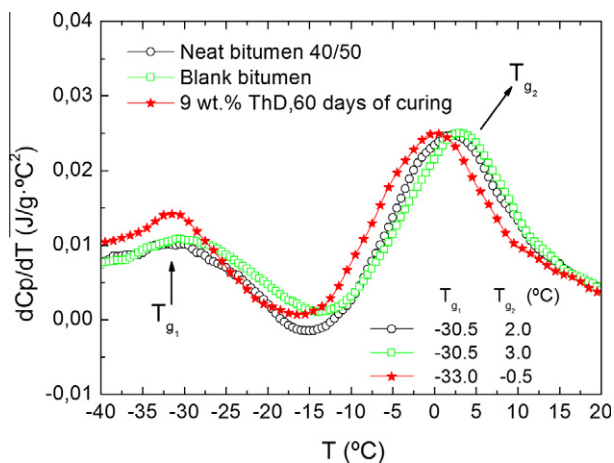
Fig. 7. Evolution of C_p derivative obtained by MDSC with temperature, for neat bitumen 40/50 and its corresponding “blank”, and 9 wt.% ThD modified bitumen, after 60 days of curing.
