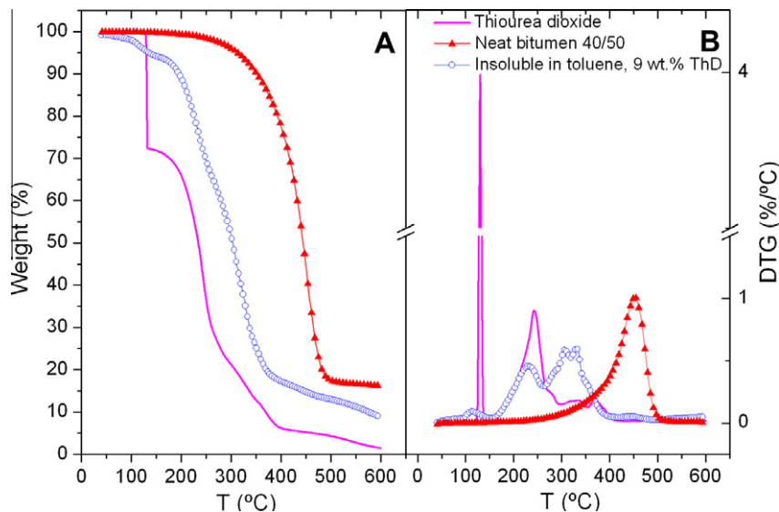
Fig. 9. Weight loss (A) and its derivative (B), between 40 and 600 °C and under N 2 atmosphere, for thiourea dioxide, neat bitumen 40/50 and the insoluble residue in toluene from 9 wt.% ThD modified bitumen after 60 days of curing.
