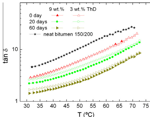
Fig. 3. Evolution of the loss tangent with temperature, for modified bitumen 150/200 samples, as a function of curing time.
