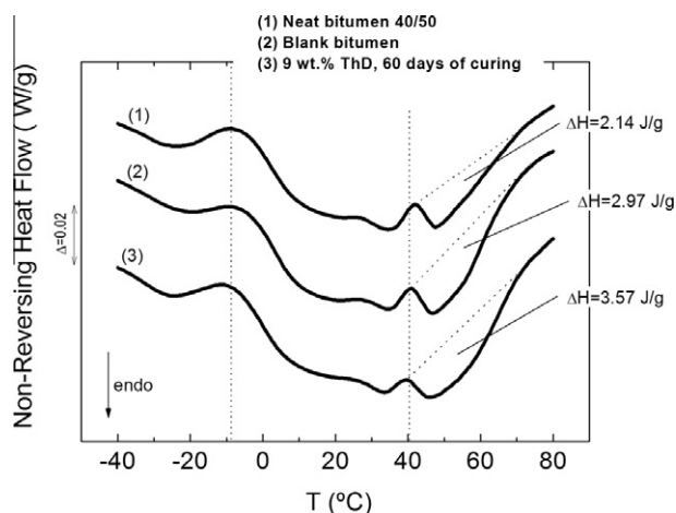
Fig. 10. Non-reversing heat flow thermograms for neat bitumen 40/50 and its corresponding "blank" and 9 wt.% ThD modified bitumen.
