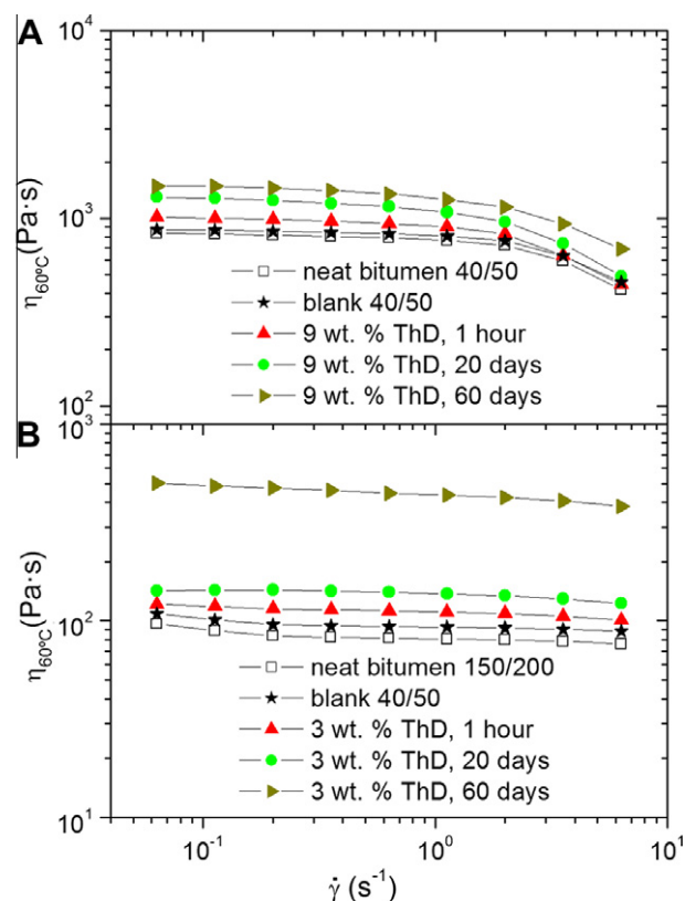
Fig. 1. Viscous flow curves, at 60 °C, for (A) 9 wt.% ThD modified bitumen 40/50 and (B) 3 wt.% ThD modified bitumen 150/200, as a function of curing time.
