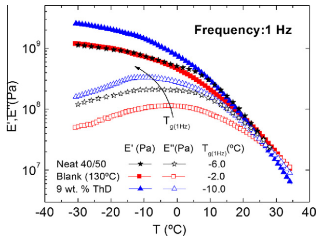
Fig. 6. Evolution of E' and E'' with temperature (temperature sweep tests) for 9 wt.% ThD modified bitumen 40/50, after 60 days of curing, and its corresponding “blank” sample.
