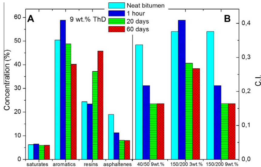
Fig. 8. Evolution of (A) SARAs fraction for 9 wt.% ThD modified bitumen 40/50 and (B) colloidal index values with curing time, for selected modified bitumen samples.
