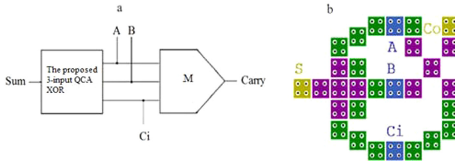
Fig. 13. The proposed robust QCA full-adder (a) logical diagram, (b) QCA layout.
