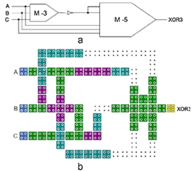
Fig. 9. The 3-input QCA XOR gate in [22] (a) logical diagram (b) QCA layout.
