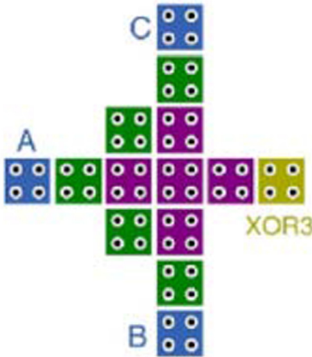
Fig. 10. The presented 3-input XOR gate in [23].
