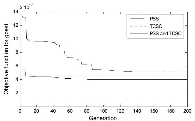
Fig. 7 Convergence of objective function for gbest
