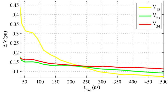
Fig. 13. Interturn voltages at the first disk for different rise times t_{\text{rise}} .
