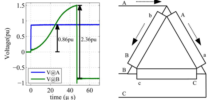
Fig. 3. Delta-connected transformer.
