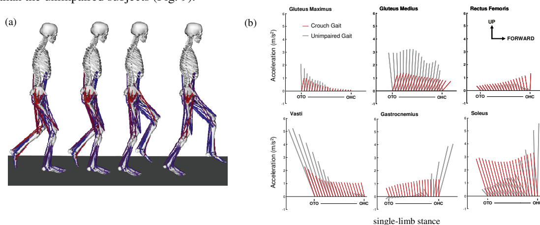
Fig. 9.(a) Crouch gait model and simulation of single-limb stance from opposite limb toe-off (OTO) to opposite limb heel-contact (OHC). (b) Muscle contributions to center-of-mass acceleration in impaired (crouch) and unimpaired gait, where each ray is the acceleration vector of the center-of-mass in the sagittal plane due to the indicated muscle. Results from Steele et al. 2010 [32]
