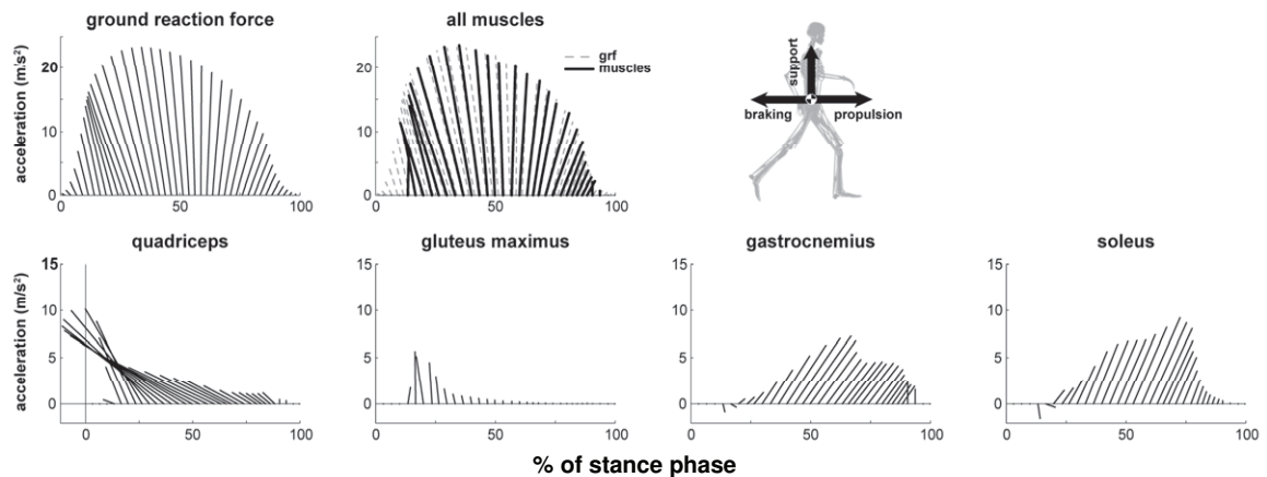
Fig. 10. Top four muscle contributions to support and propulsion during running. Muscle contributions are to center-of-mass acceleration where each ray is the acceleration vector of the center-of-mass in the sagittal plane due to the indicated muscle. Results from Hamner et al. 2010 [18]
